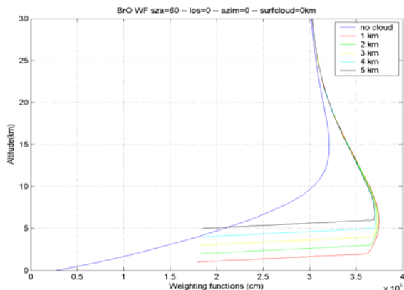
Fig. 4. BrO weighting functions for different cloud altitudes. The curves are associated to completely cloudy scenes at different altitudes.
