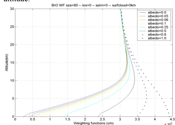
Fig.3. BrO weighting functions for different ground albedo. Calculations are for a solar zenith angle of 60° in a pure nadir viewing geometry.
