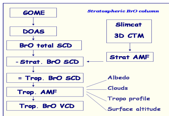
Fig. 1. Overview of the tropospheric BrO retrieval algorithm
