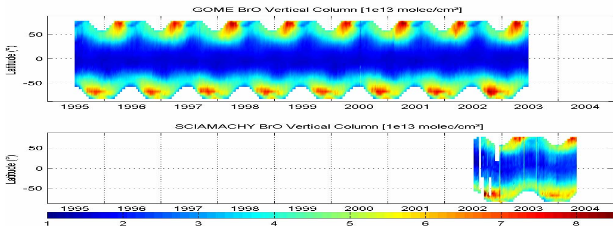
Fig. 8. GOME and SCIAMACHY BrO vertical column distributions.
