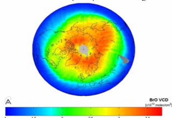
Fig. 2. SLIMCAT stratospheric BrO distribution for March 2001.
