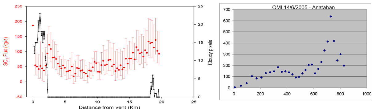
Figure 9: Results of the flux calculation around Anatahan on the 14 June 2005. The fluxes are plotted as a function of the distance from the volcano for ASTER on the left panel and from OMI on the right panel.
